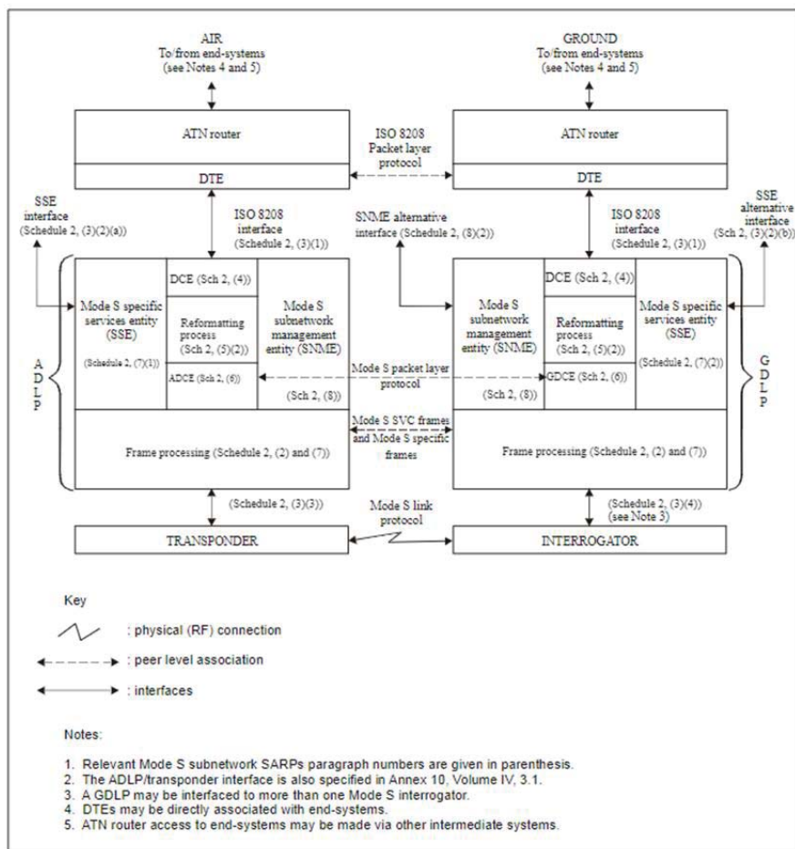
Functional elements of the Mode S subnetwork
