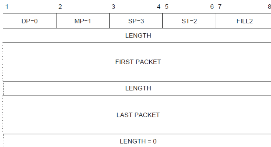
Figure 6-20. MULTIPLEX packet
