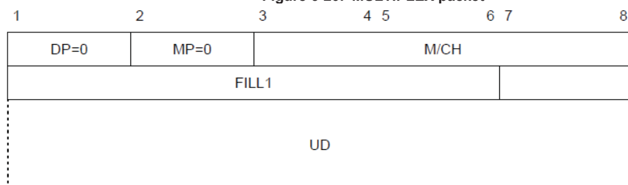
Figure 6-21. SHORT FORM MSP packet
