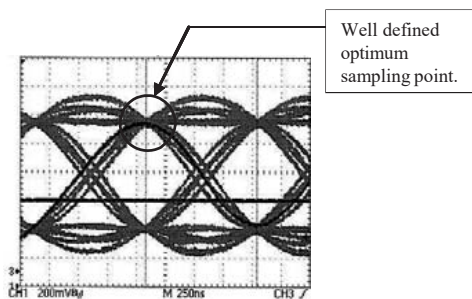
Figure 15-3. Ideal eye diagram
