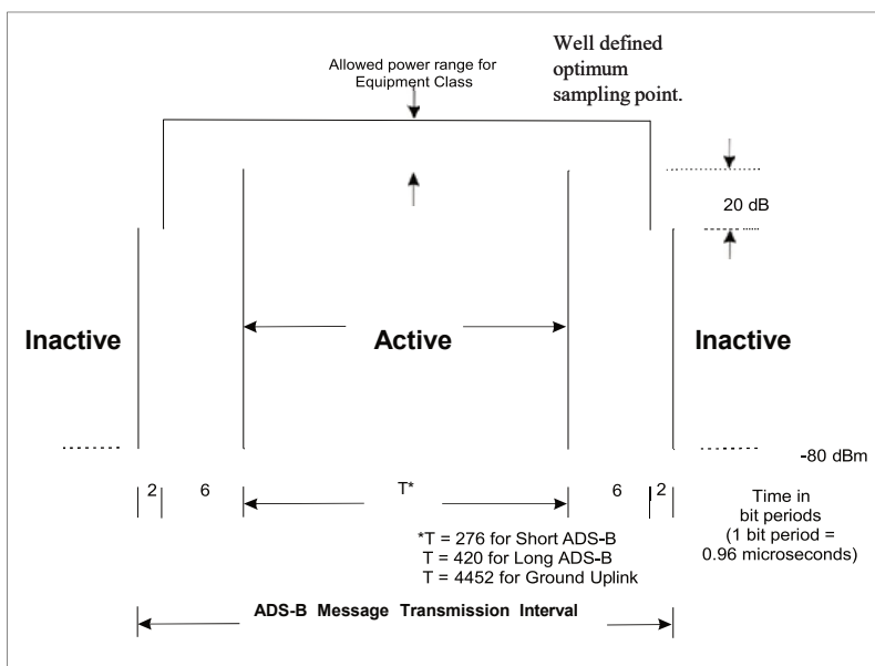
Figure 15-2. Time/amplitude profile of UAT message transmission
