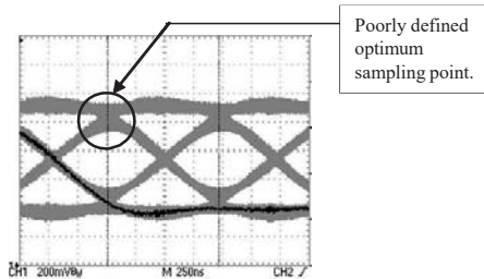
Figure 15-4. Distorted eye diagram
