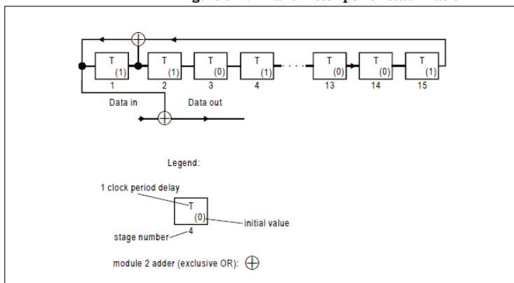
Figure 9-2. PN-generator for bit scrambling sequence
