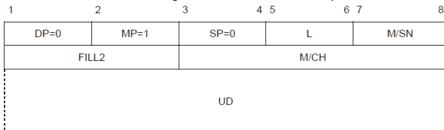
Figure 6-22. LONG FORM MSP packet
