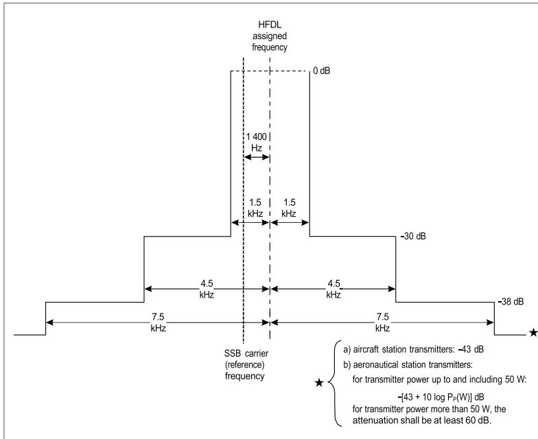
Figure 14-1. Required spectrum limits (in terms of peak power) for HF DL aircraft and ground station transmitters
