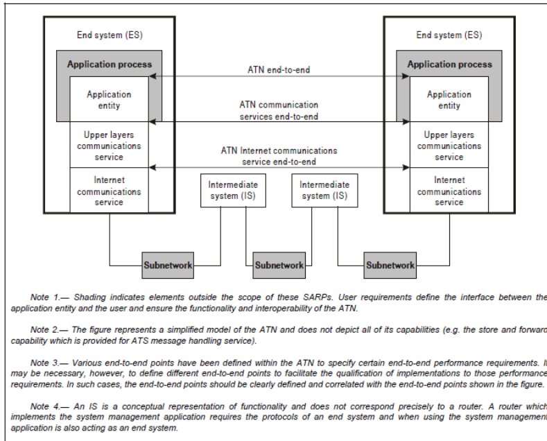
Figure 1-1. Conceptual model of the ATN
