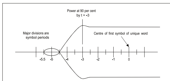
Figure 9-1. Transmitter power stabilization
